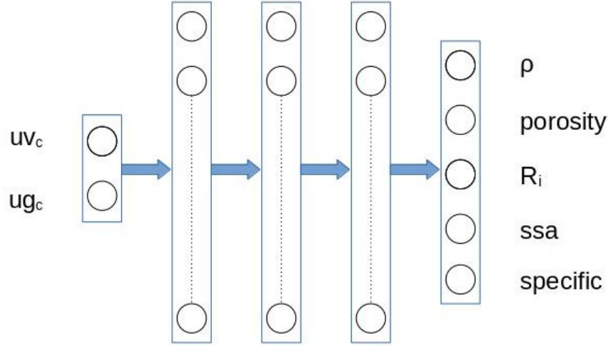
Fig. 1. MLP Regressor Architecture
